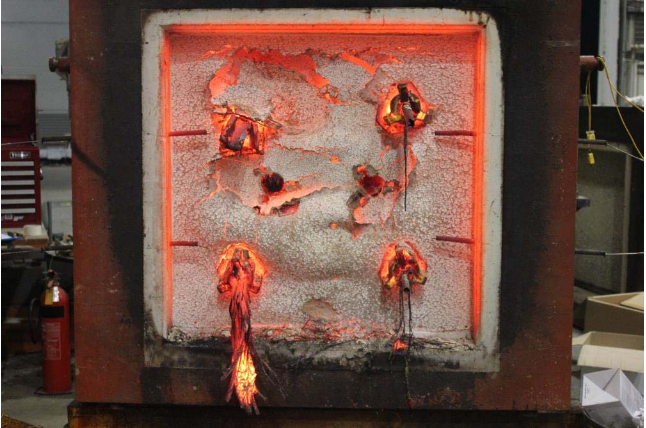
PHOTOGRAPH 16 – EXPOSED FACE OF SPECIMENS AT CONCLUSION OF TESTING
