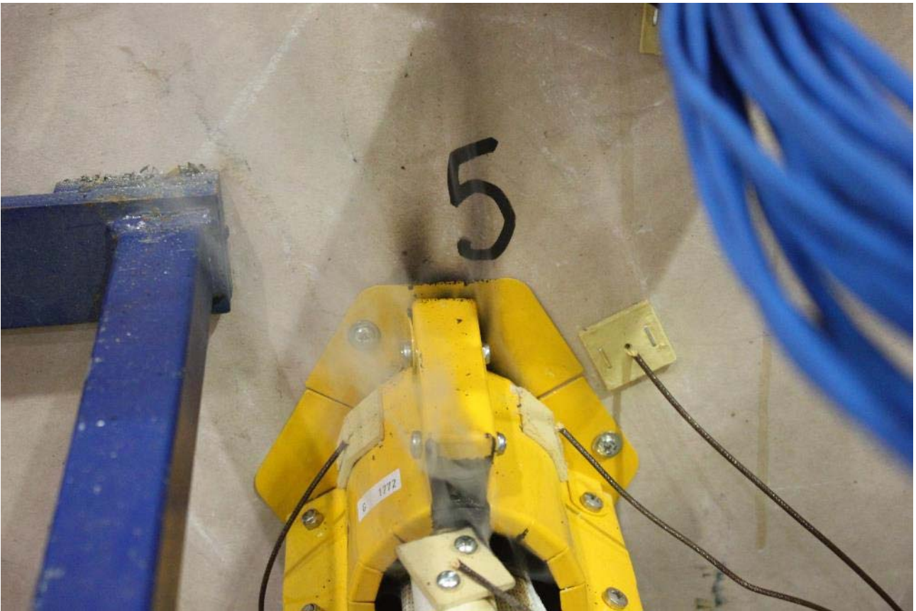
PHOTOGRAPH 11 – SPECIMEN 5 AFTER 75 MINUTES OF TESTING
