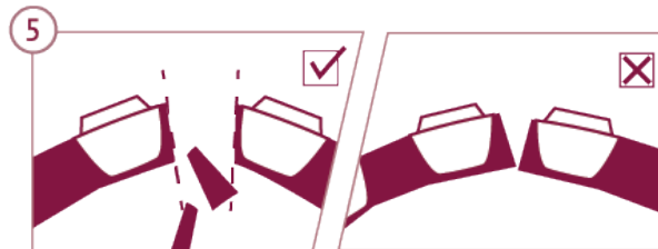
5 Trim the intumescent strip on an angle
