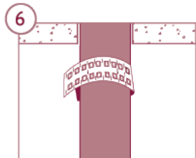
6 Wrap collar around pipe
