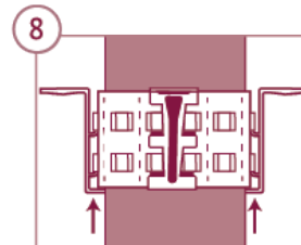
8 Add additional brackets spaced out evenly and fix (see Table 4)
