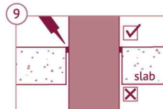
9 Seal annular gap between the slab and pipe only on top as required (see Table 3)
